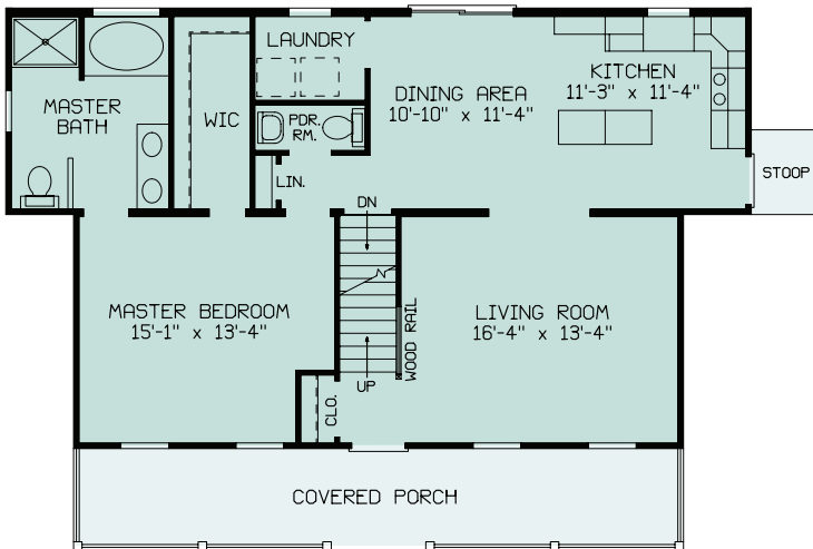
YORKTOWN PLAN A 44'-0 x 32'-0 1033 SQ. FT.
