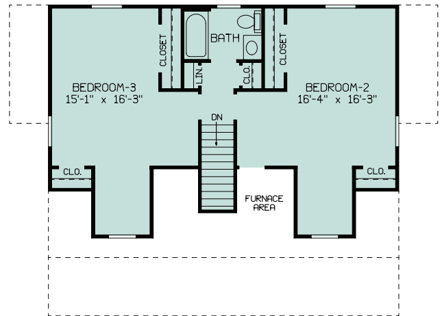
YORKTOWN PLAN A 36'-0 x 32'-0 736 SQ. FT.
