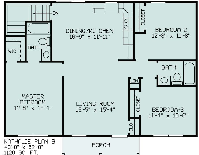
Nathalie B 40' x 32' 1120 Sq. Ft.
