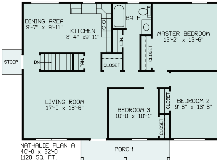
Nathalie A 40' x 32' 1120 Sq. Ft.
