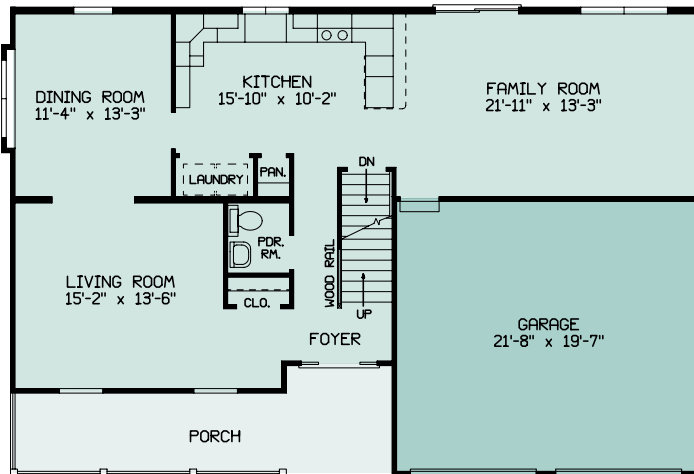
SAVANNAH PLAN D 50'-0" x 34'-0" 1078 SQ. FT.
